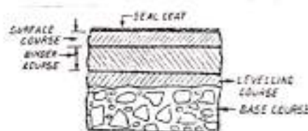
SECTION SHOWING COMPONENTS OF A BITUMINOUS SURFACE
